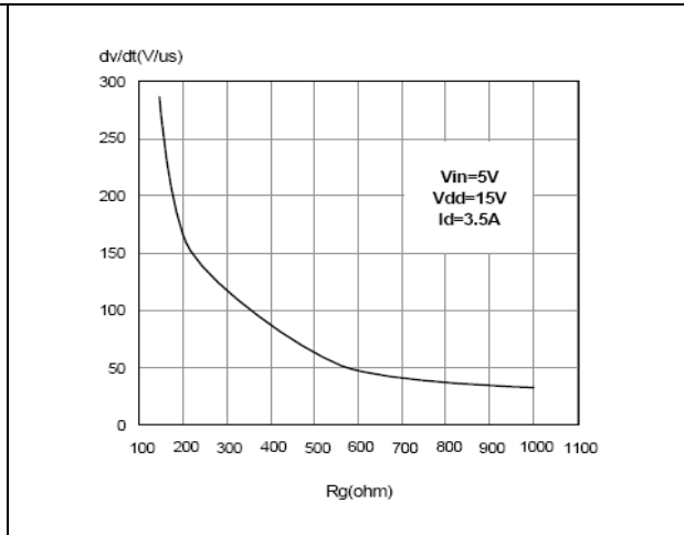
Figure 42. Turn-off drain source voltage slope ( V_{in}=5V )
