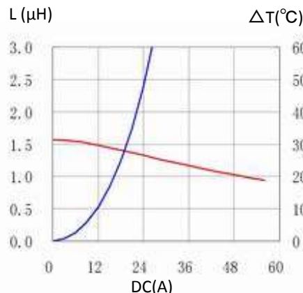
6. 125CDMCCDS-1R5MC
