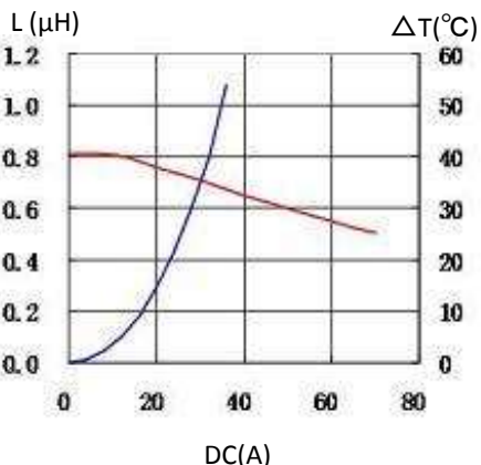
4. 125CDMCCDS-R82MC
