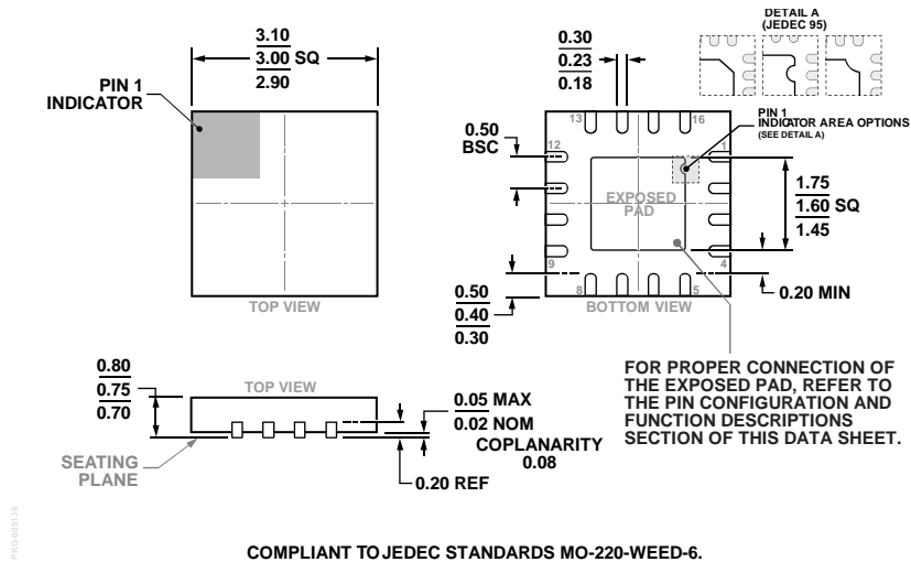
Figure 49. 16-Lead Lead Frame Chip Scale Package [LFCSP] 3 mm × 3 mm Body and 0.75 mm Package Height (CP-16-22)
