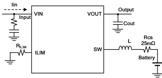
Figure 7. Input current limit setting circuit
