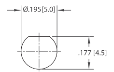
MOUNTING HOLE P
