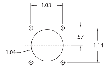
MOUNTING HOLE AJ
