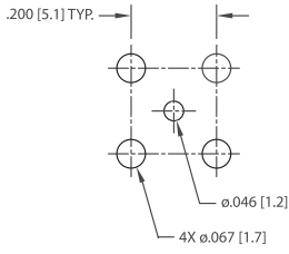
MOUNTING HOLE U
