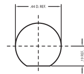
MOUNTING HOLE AB
